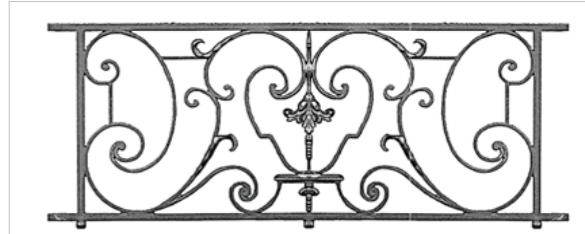
MR HT1: 580mm LG1: 1570mm LG2: 1385mm
