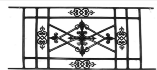
MM HT1: 520mm HT2: 440mm HT3: 353mm LG1: 1080mm LG2: 863mm LG3: 685mm LG4: 436mm
